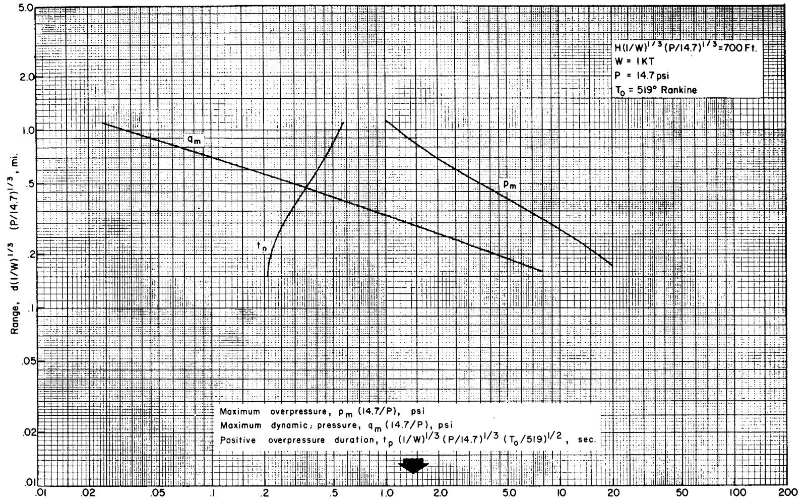
Fig. 2.8—Scaled blast parameters for a scaled height of burst of 700 ft as a function of scaled range. These are plots of Eqs. 2.54, 2.56, and 2.58 given in Table 2.8.
